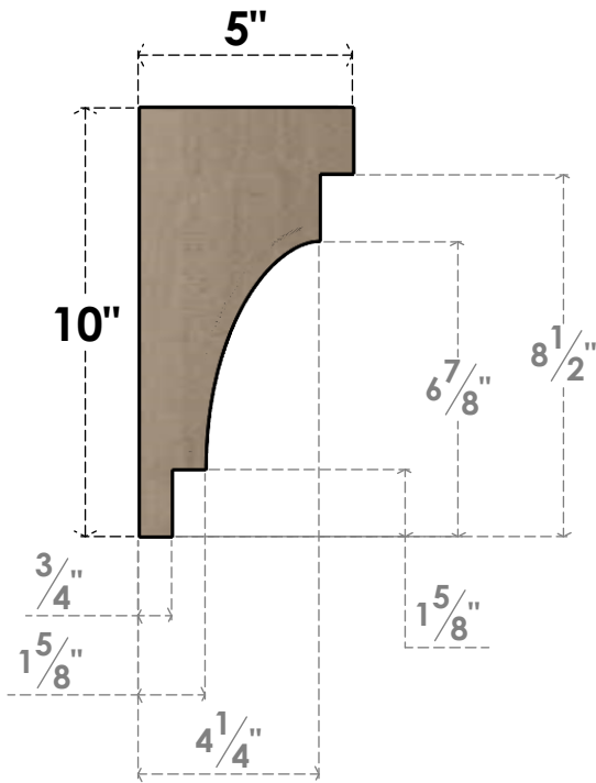
SIDE PROFILE
